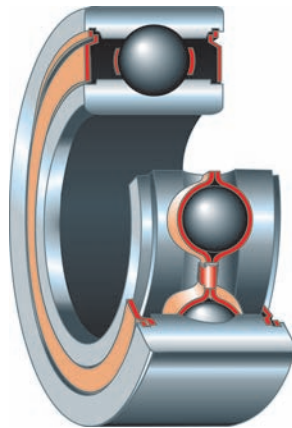
Deep Groove Shielded
