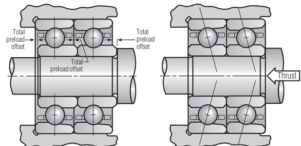
Fig. 11. DT mounting.
