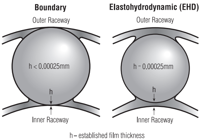
Fig. 14. Lubrication regimes.
