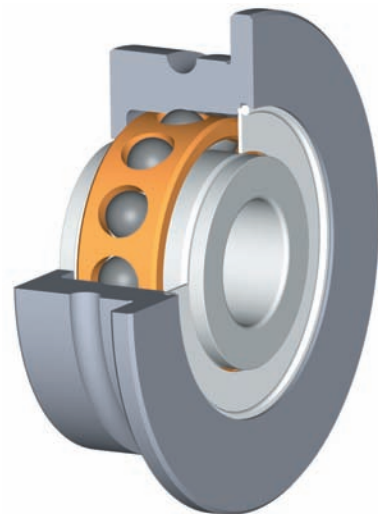
TMP Flange Bearing with Integral Damping Ring Groove
