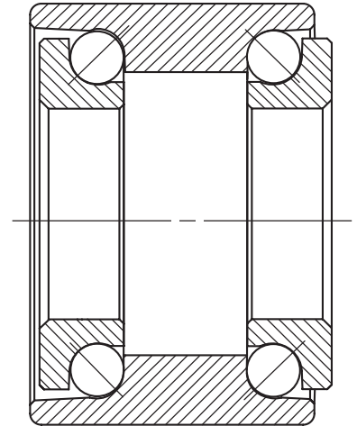
Double-Row Accessory Bearing
