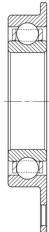
Flanged Deep Groove Gear Box Bearing
