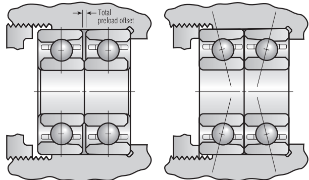
Fig. 10. DF mounting.
