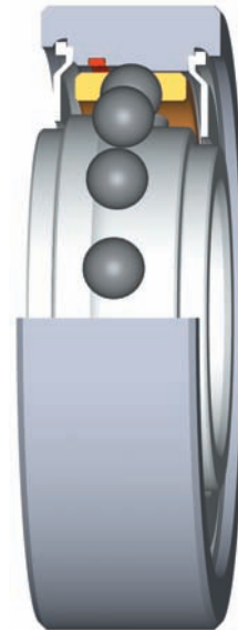
Dry Pump Bearing with Grease Reservoir
